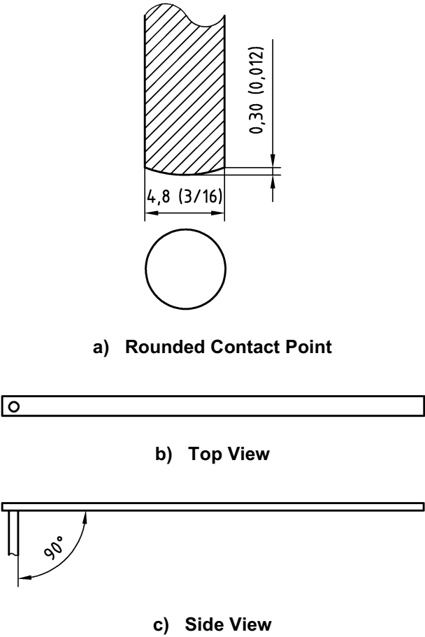
Figure D.25—Example of a 90° Hook-type Tool
