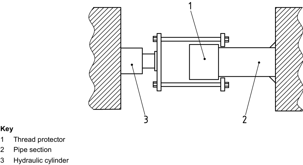
Figure D.28—Stripping Test Apparatus
