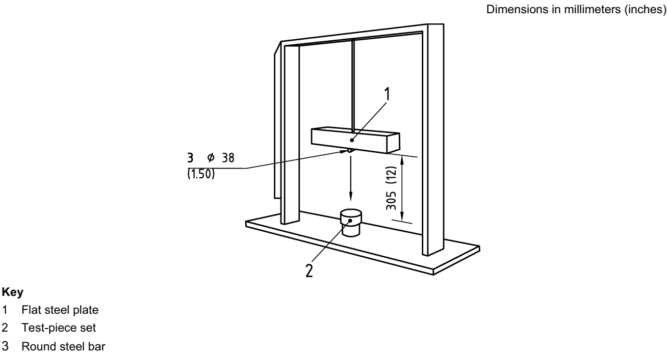
Figure D.26—Axial Impact Test Apparatus
