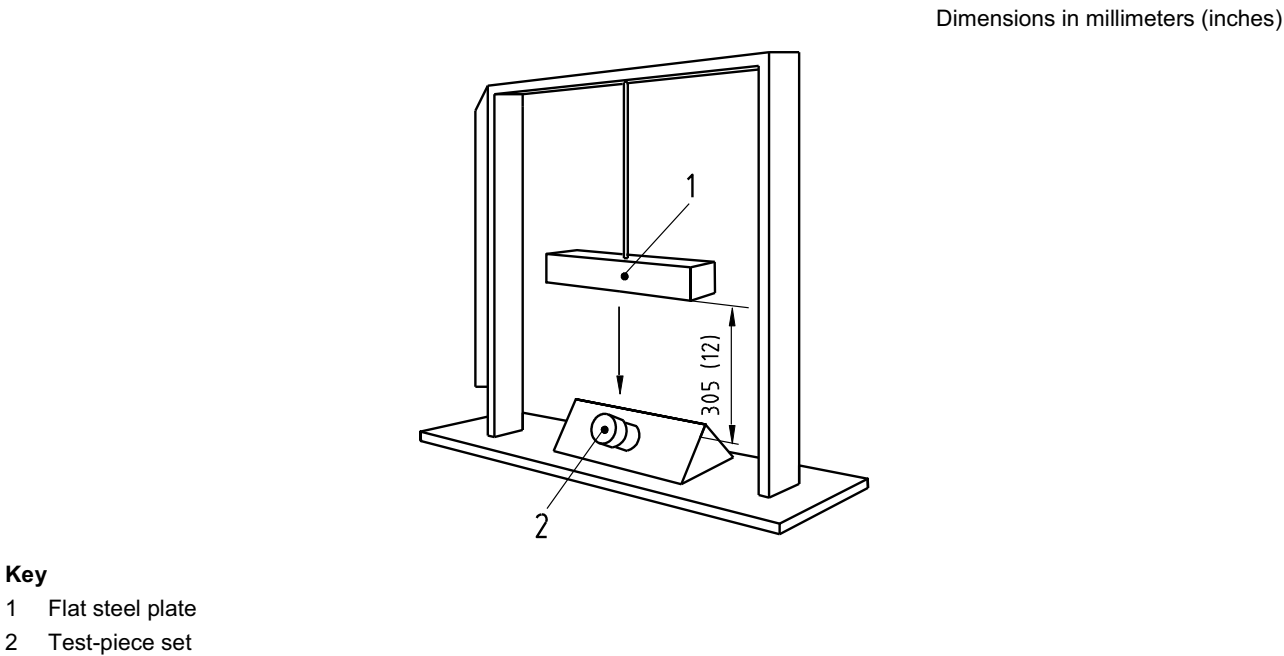
Figure D.27—45° Impact Test Apparatus
